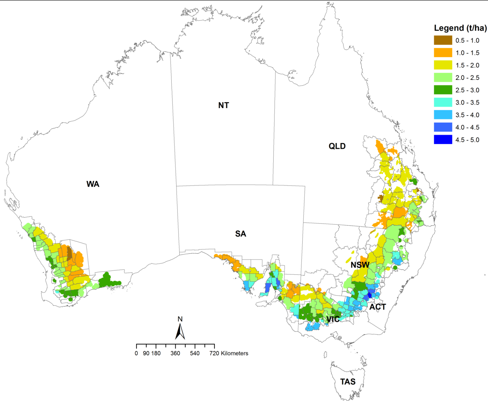
Simulated shire wheat yield long-term median (OZ-Wheat MII, from 1901-2017)
